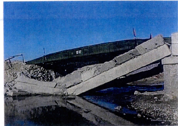
photo 2. Blown bridge with MTU-20 across the blown span on New Kabul Road (5.8km). River depth ranges from 3 feet to 1 foot.
